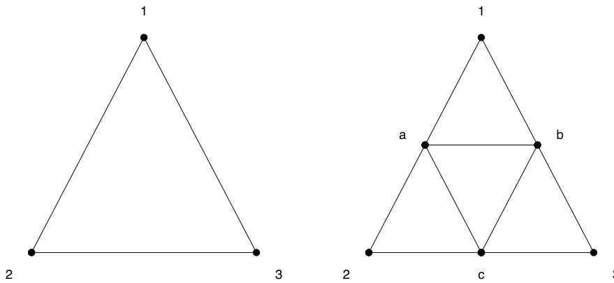
Figure 2. Labelling of sites used for \mathcal{G}_0 and \mathcal{G}_1 .
